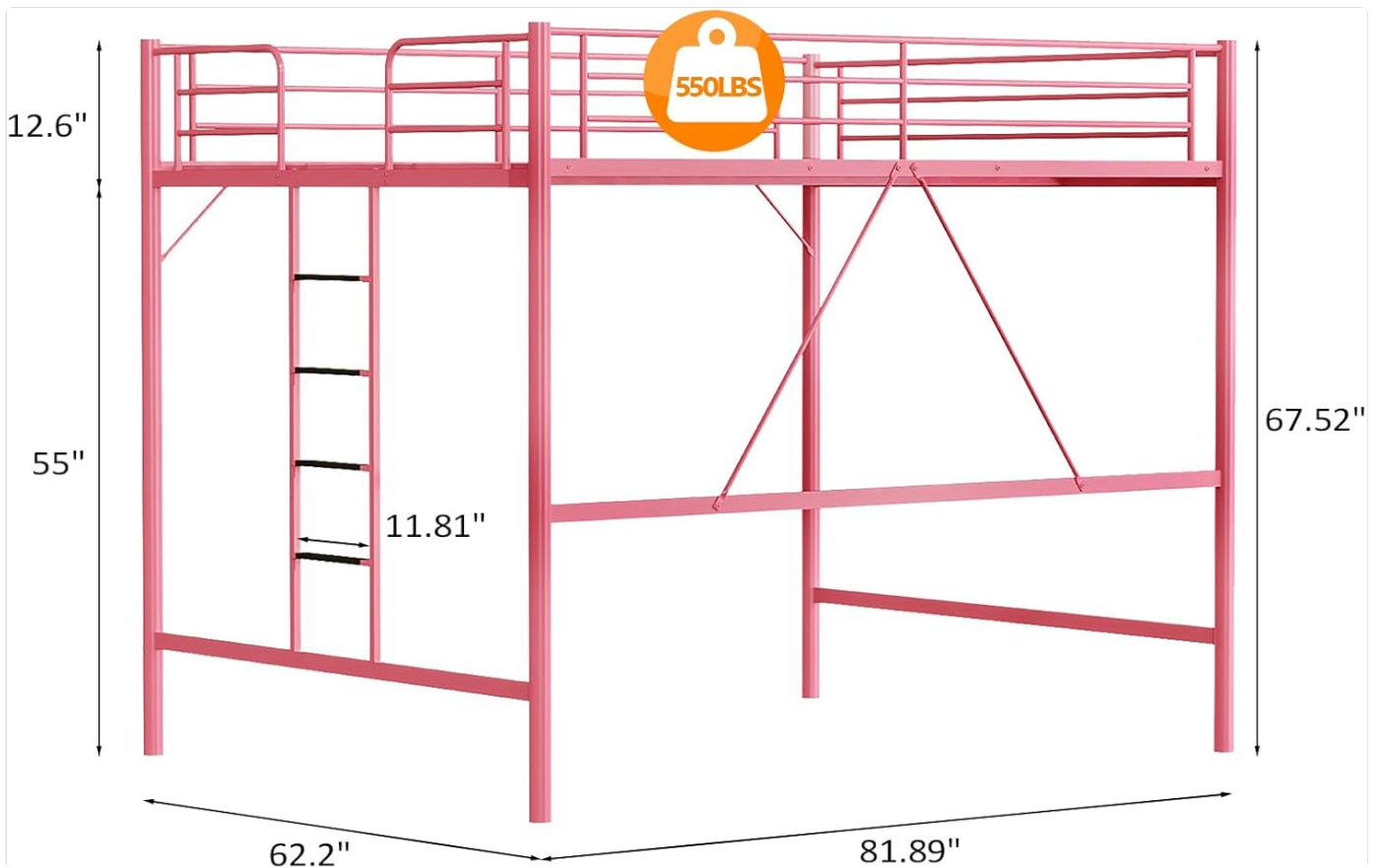
Figure 8.1: Dimensional overview of the VINGLI Pink Queen Loft Bed.
