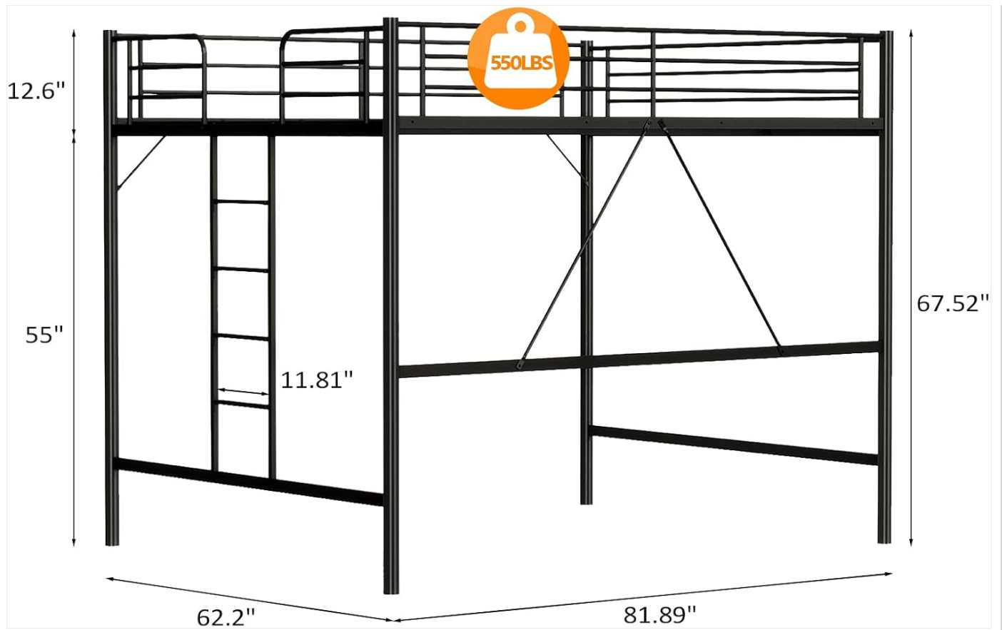
Dimensional overview of the VINGLI Queen Loft Bed.
