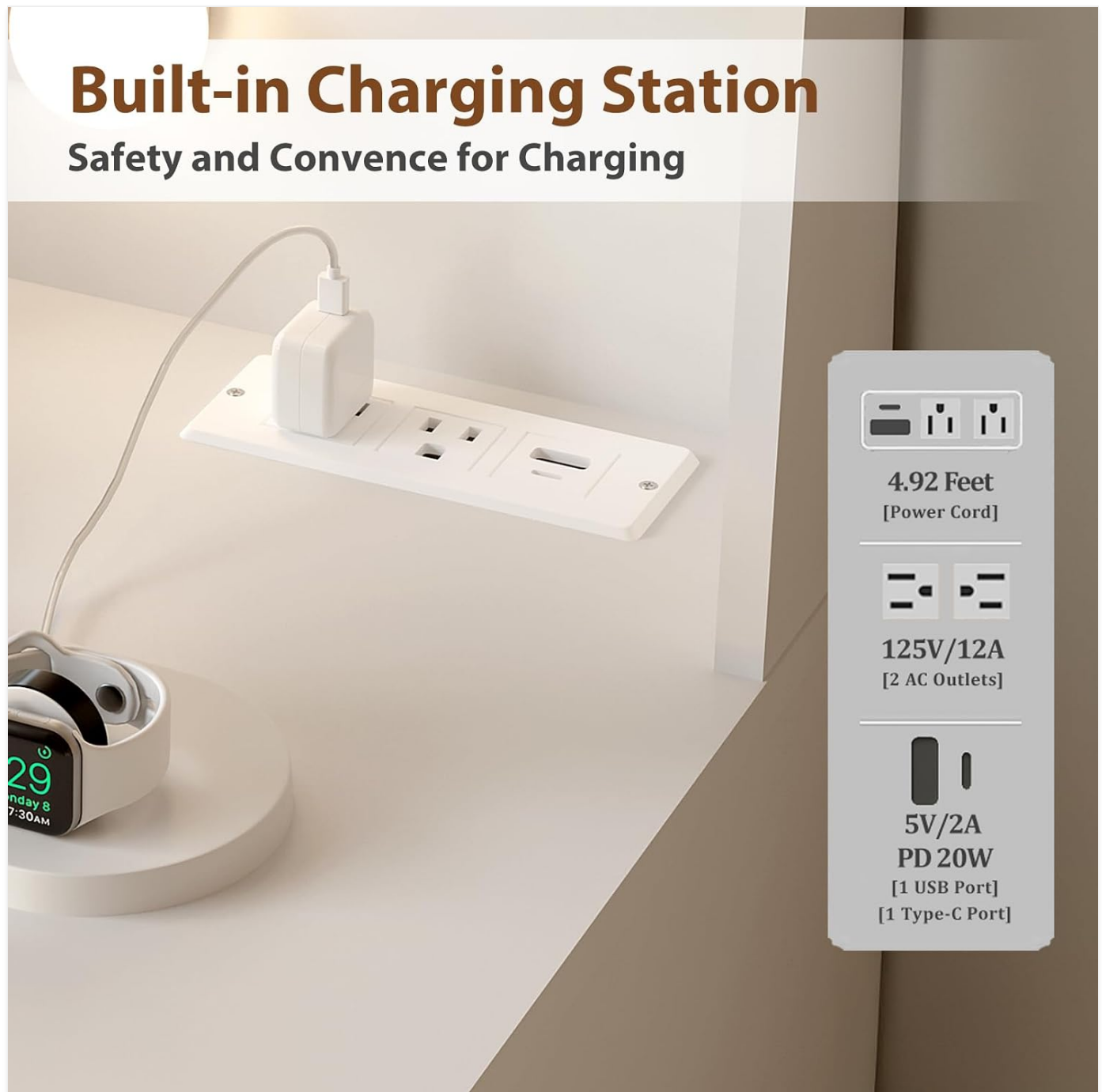
Figure 5.2: The integrated charging station provides convenient power access for various devices.
