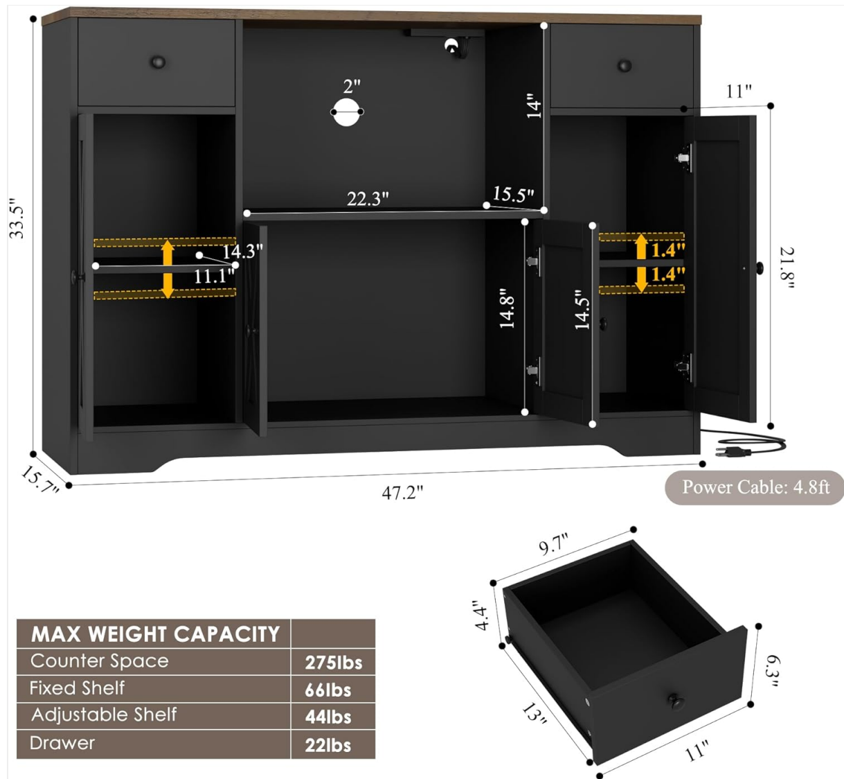
Figure 1: Detailed dimensions and weight capacities of the cabinet components.
