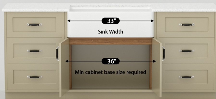
Image 4.2: Cabinet base size requirement for sink installation.
