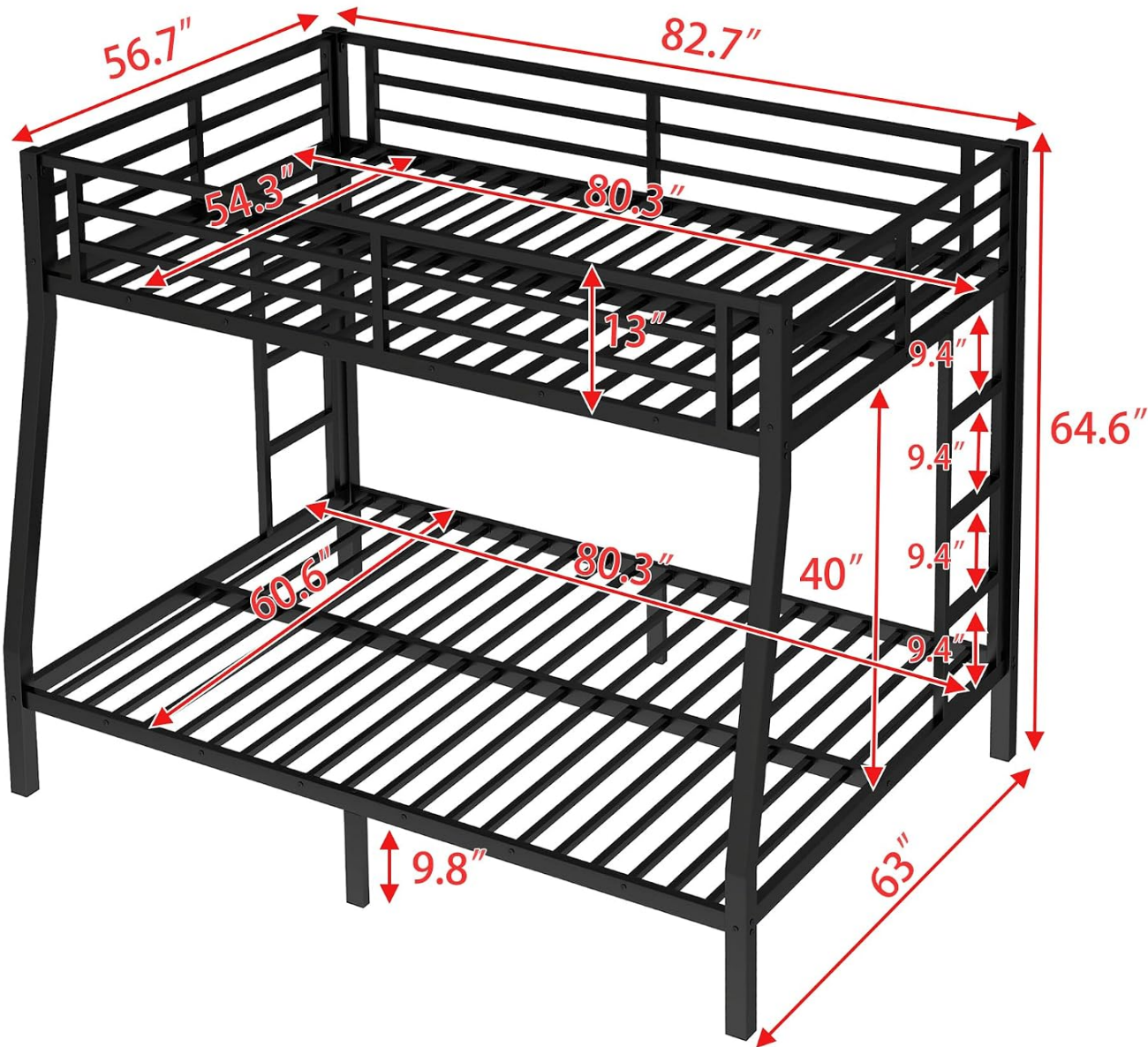
Image: A technical diagram illustrating the precise dimensions of the Bellemave Full XL Over Queen Bunk Bed in inches.
