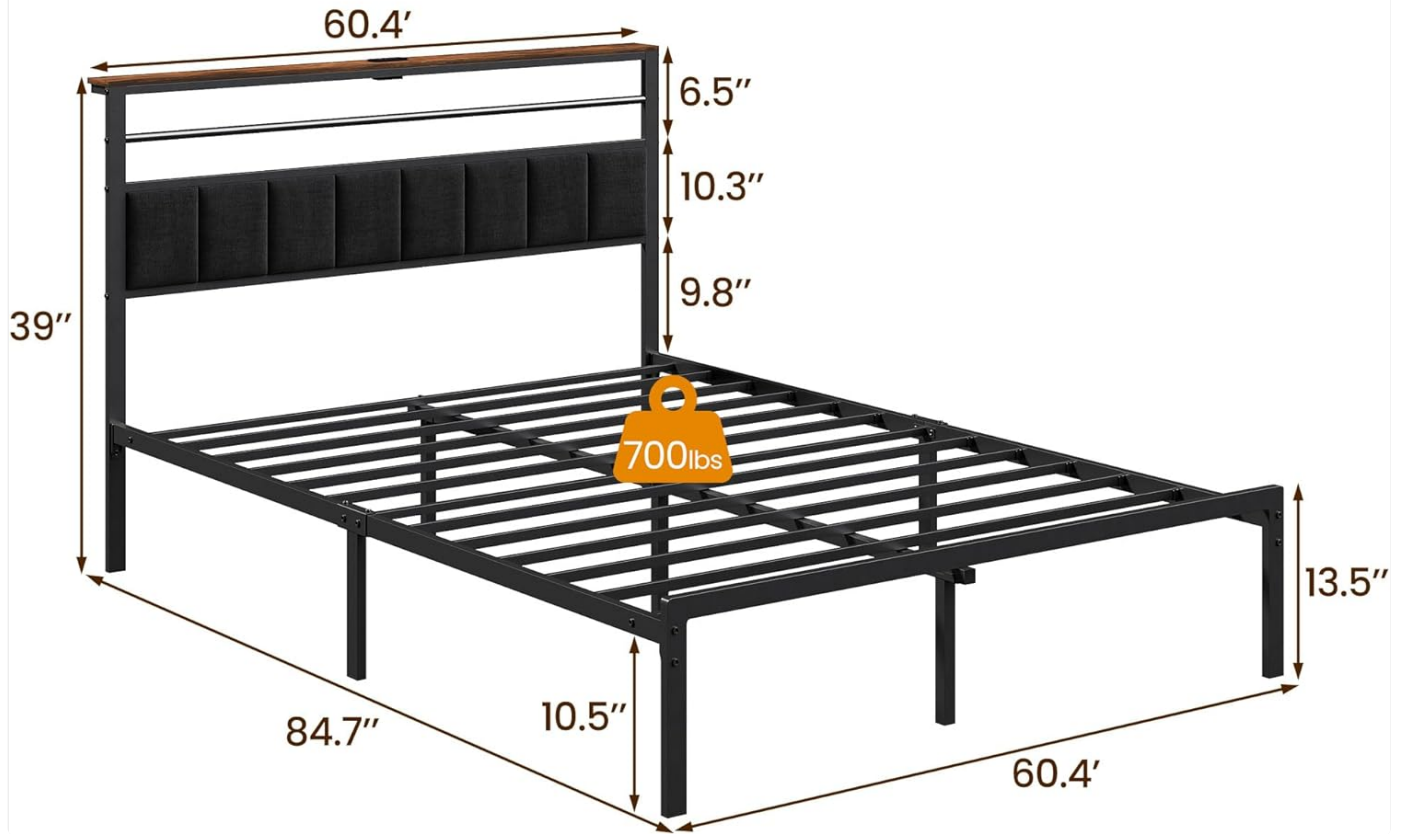
Image: Detailed product dimensions for the RoyalCraft ZBBD003 Queen Bed Frame, including length, width, and height measurements.
