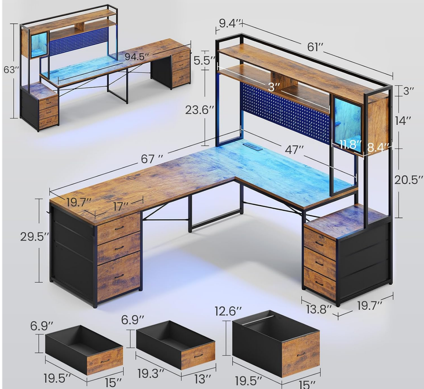
Image: A diagram illustrating the detailed dimensions of the desk, hutch, and drawer units, useful for planning your space.
