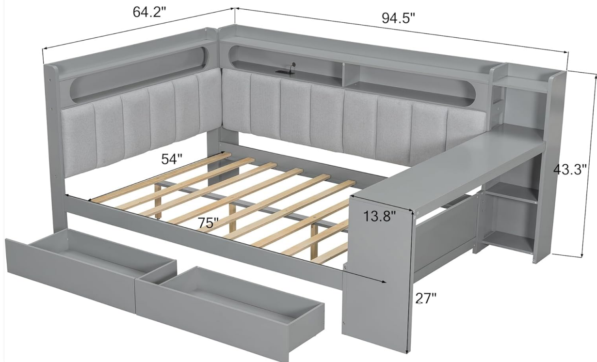
Image 2: Dimensional diagram of the VilroCaz Full Size Daybed Sofa Bed, showing overall dimensions of 94.5\"L x 64.2\"W x 43.3\"H, bed dimension 75\"x 54\", and desk height 27\".
