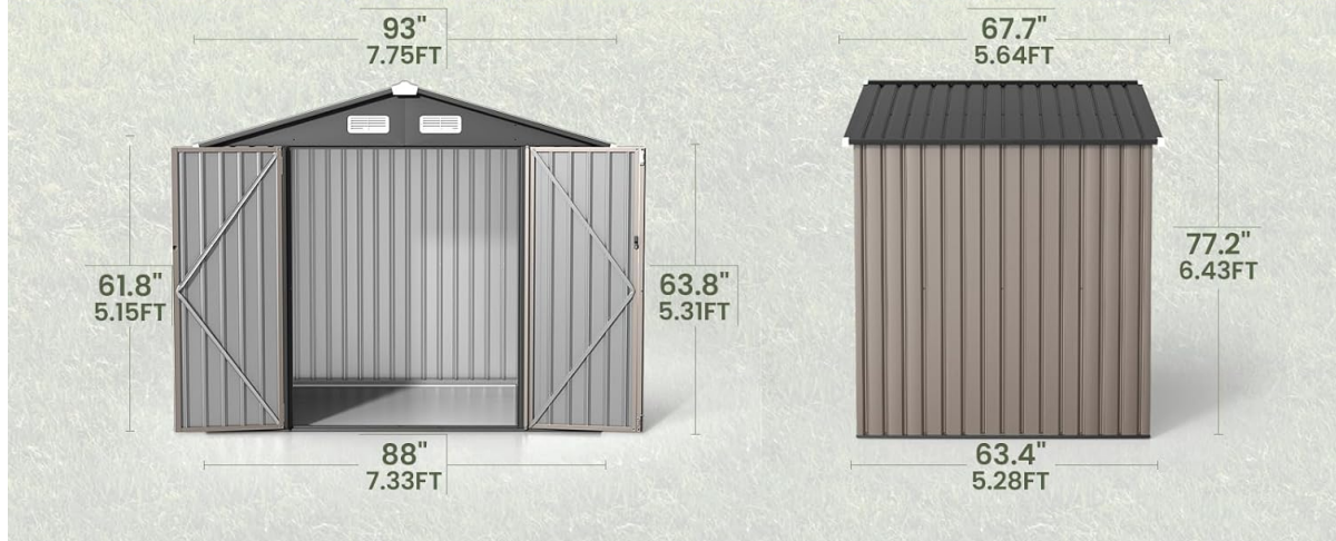
Image: Detailed dimensions of the GVDV 8x6 FT Outdoor Metal Storage Shed.
