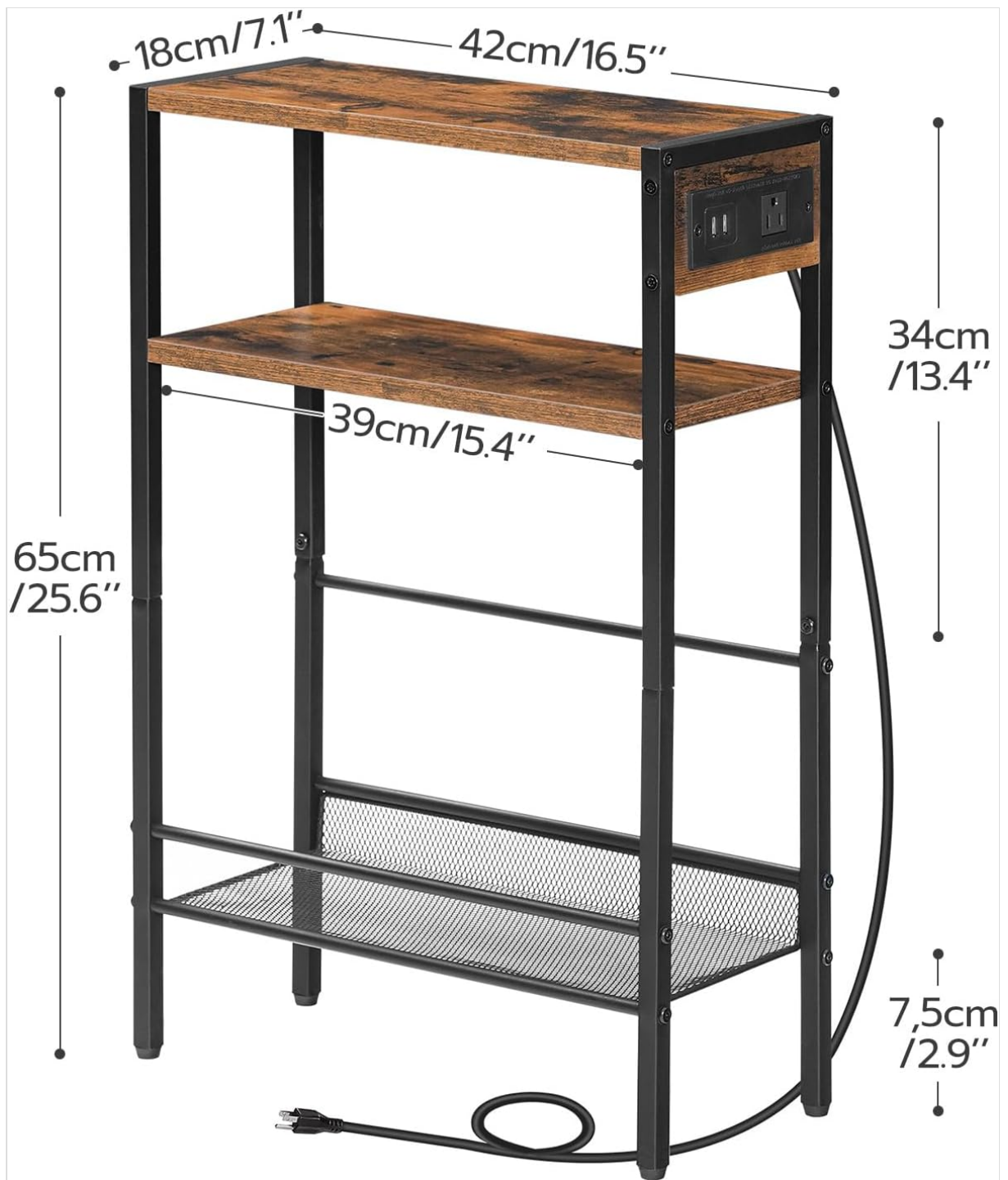
Image: Detailed dimensions of the side table, including length, width, and height measurements.
