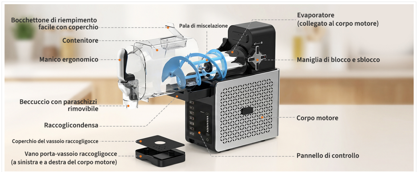
Figure 1: Exploded view of the Garvee FS-201 Slush Machine, showing the main components such as the filling port with lid, mixing paddle, container, ergonomic handle, removable splash-proof spout, condensation collector, drip tray cover, drip tray holder, motor body, and control panel.
