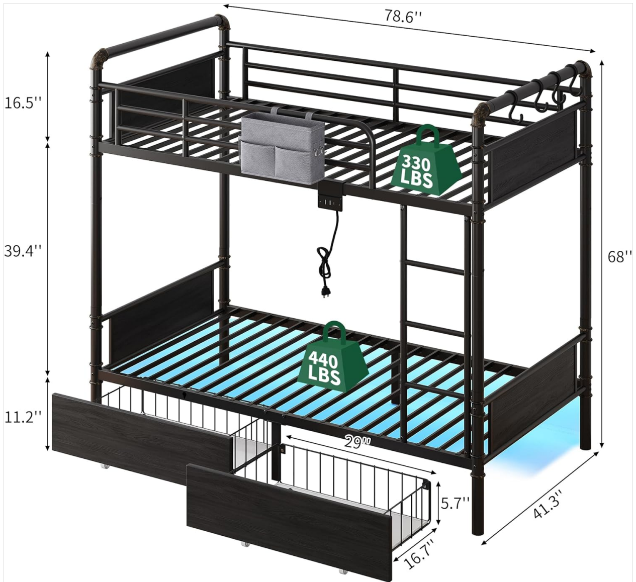
Image 3.1: An annotated diagram illustrating the dimensions and key components of the bunk bed, including storage drawers and weight capacities.
