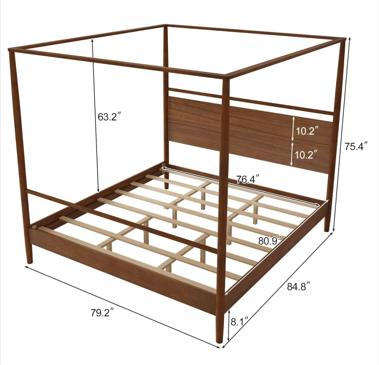
Image 3: Detailed dimensional drawing of the King Size GDFStudio Darnal Canopy Platform Bed, indicating overall length, width, and height measurements.
