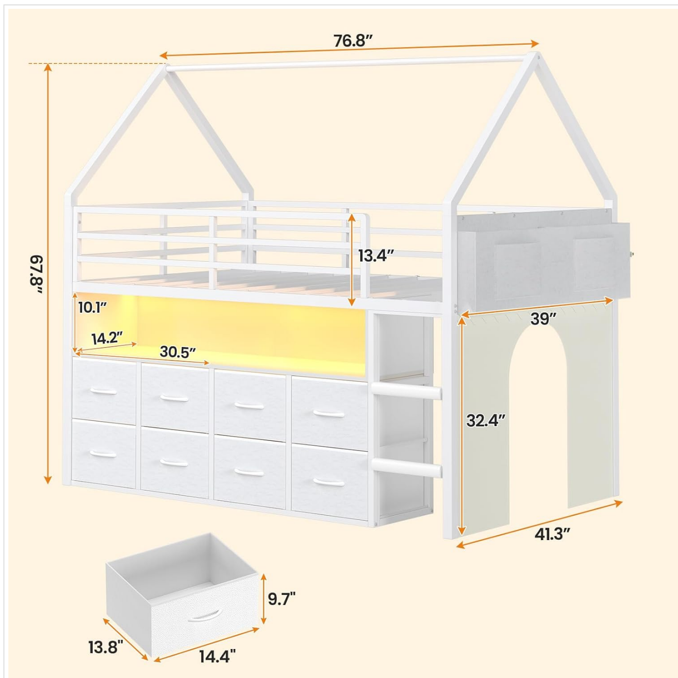
Image: Detailed dimensions of the BTHFST Low Loft Bed, including overall length (76.8"), width (41.3"), height (67.8"), guardrail height (13.4"), and drawer/shelf dimensions.
