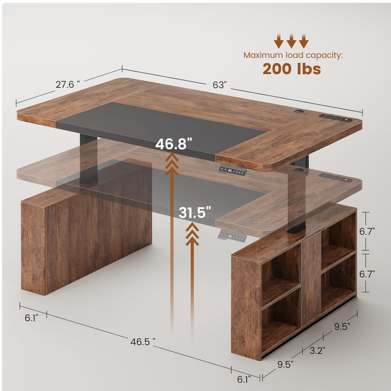
Image 2.1: Dimensional overview of the desk, indicating a maximum load capacity of 200 lbs.
