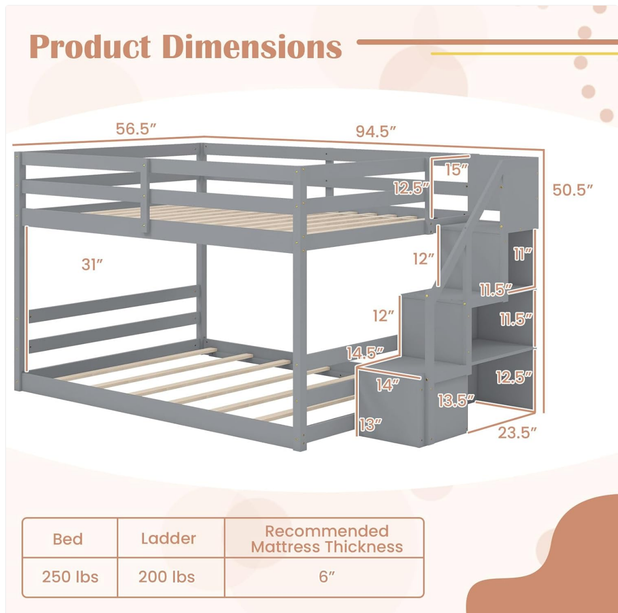
Image: Diagram illustrating the dimensions of the Giantex Full Over Full Bunk Bed, including length, width, height, and staircase step measurements. Recommended mattress thickness is 6 inches.
