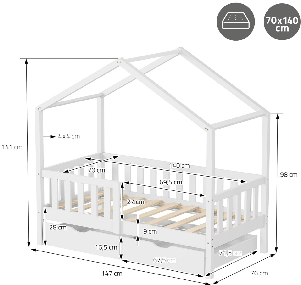
Image 3.2: A technical diagram providing precise measurements of the bed frame, including overall dimensions, mattress area (70x140 cm), and drawer height.
