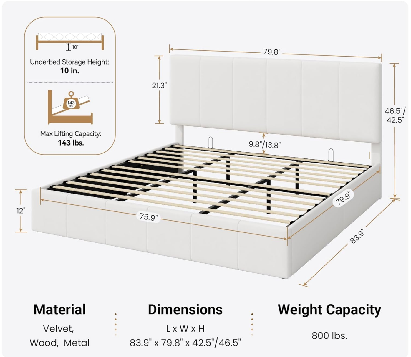
Figure 8.1: Detailed dimensions and capacities of the King Size Lift Up Storage Bed Frame.
