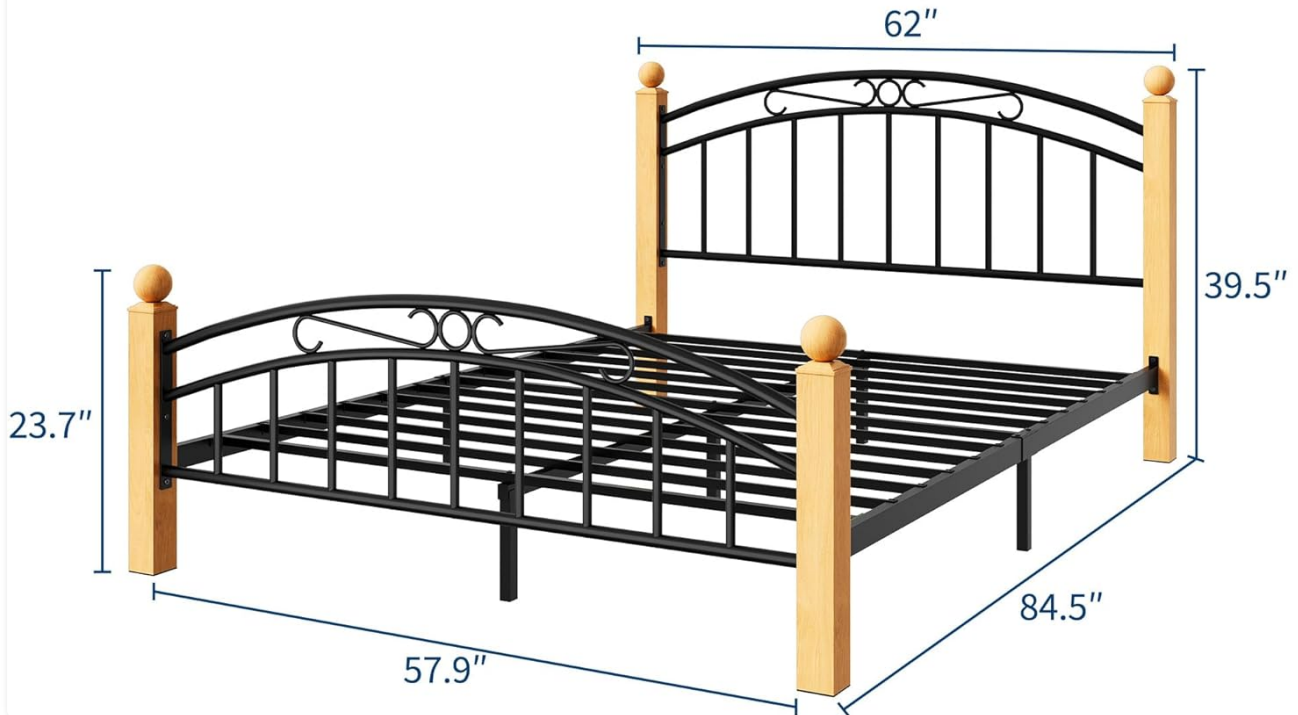
Image: A detailed diagram illustrating the Queen size dimensions (L×W×H: 84.5"×62"×39.5"), maximum capacity (800 lbs), and recommended mattress thickness (8-12 inches).
