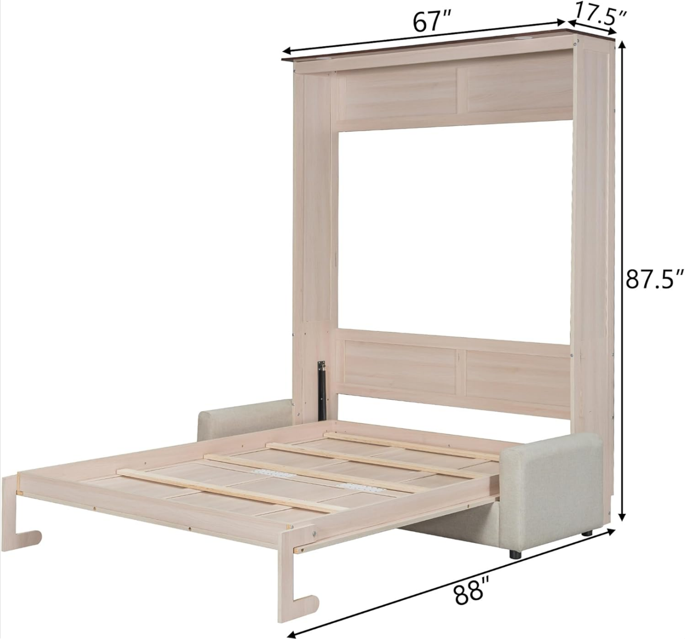
Image: Diagram illustrating the key dimensions of the DERCASS Murphy Cabinet Bed, including overall length, width, and height.
