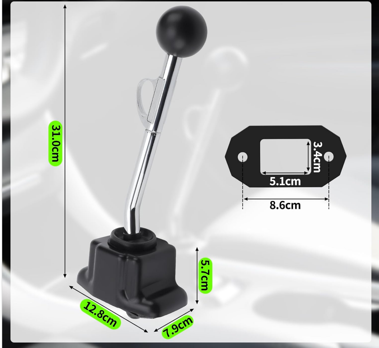
Image: Detailed product dimensions for the trigger shifter.
