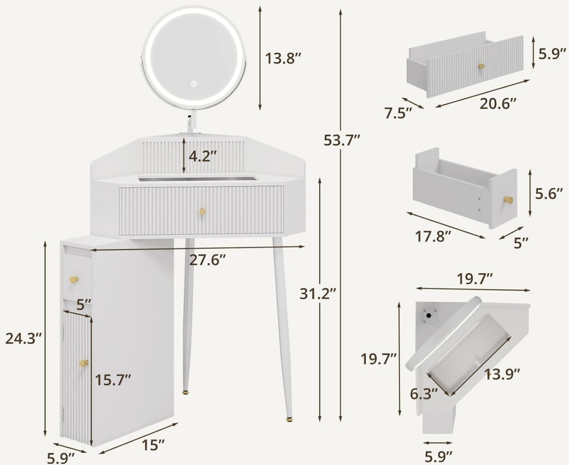
Figure 4.1: Diagram showing product dimensions and individual components. This image illustrates the various parts of the vanity desk and their respective measurements, aiding in component identification.
