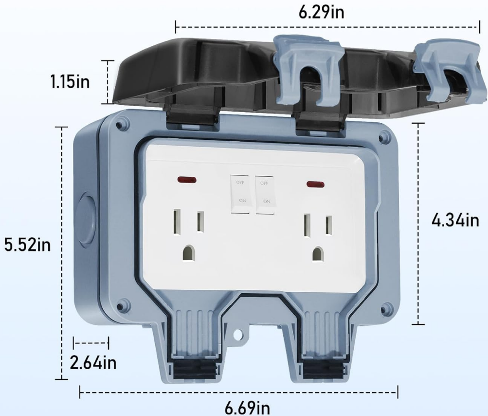
Image: Diagram showing the dimensions of the BSEED Outdoor Outlet Box, including width, height, and depth measurements.
