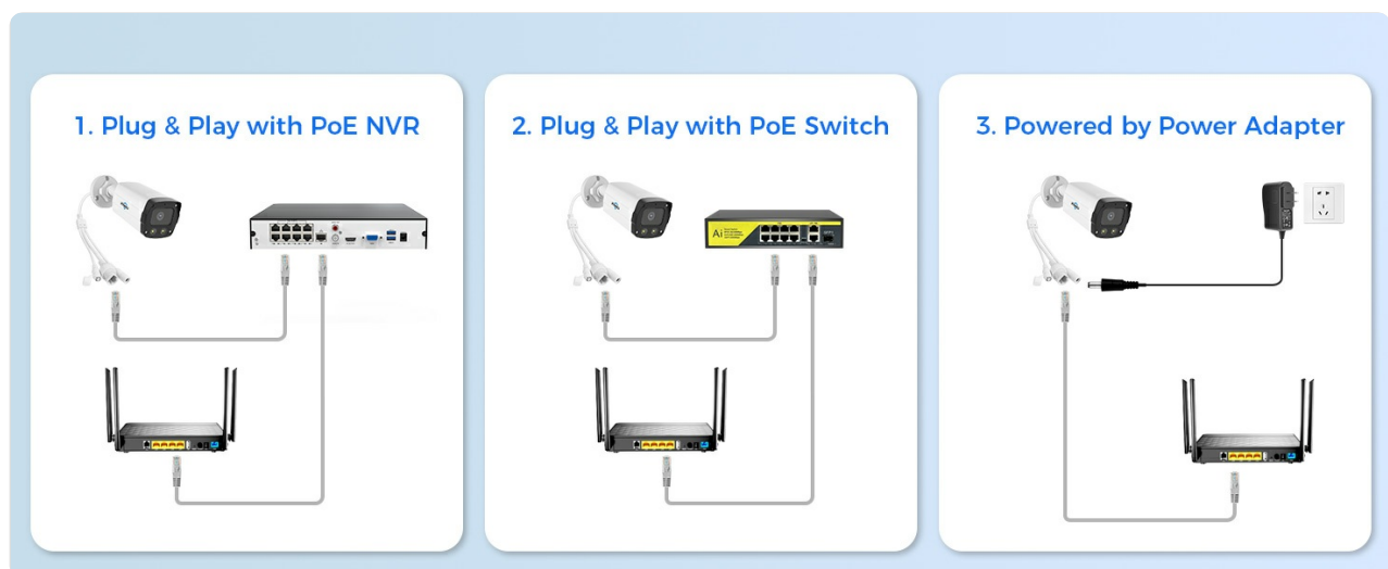
Image: Connection Methods for Hiseeu PoE Camera. This diagram illustrates connecting the camera via a PoE NVR, a PoE switch, or a standard power adapter.
