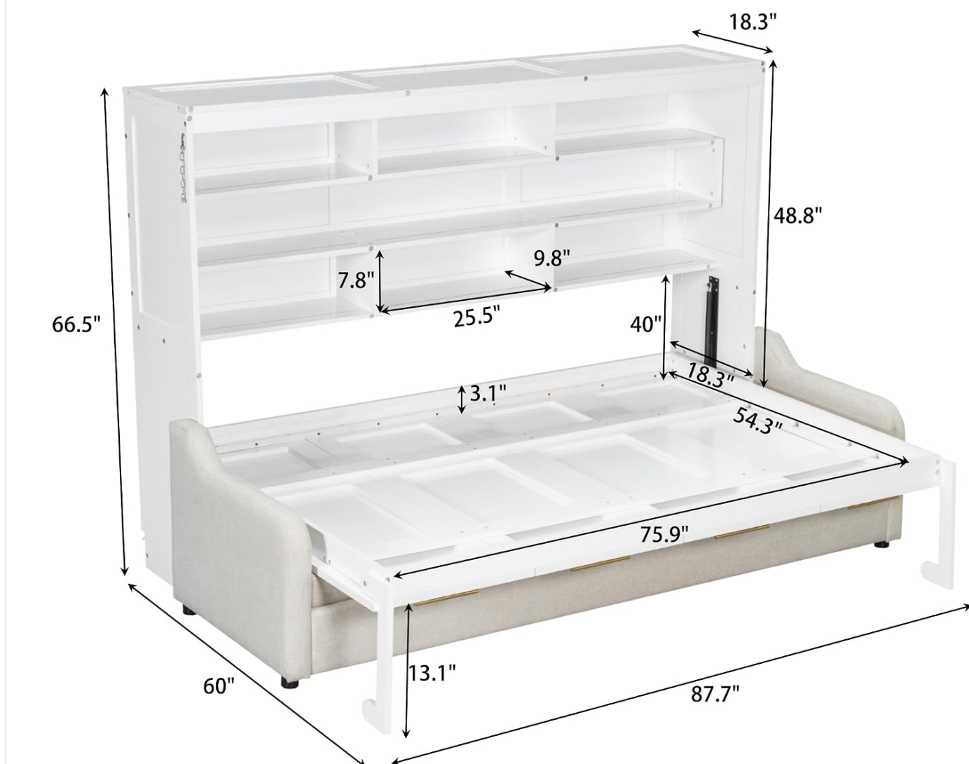
Figure 1: Detailed dimension diagram of the DERCASS Murphy Cabinet Bed, showing measurements in inches for the cabinet, bed frame, and sofa components.
