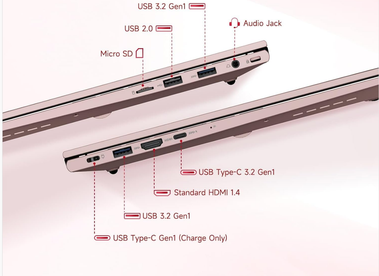
Image 3.1: Overview of the laptop's multiple ports for enhanced connectivity.
