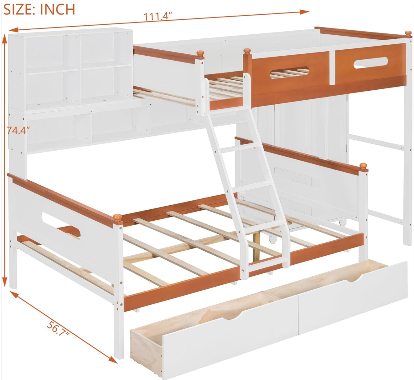
Image: A diagram illustrating the overall dimensions of the Merax Twin Over Full Wooden Bunk Bed: 111.4 inches in length, 56.7 inches in width, and 74.4 inches in height.
