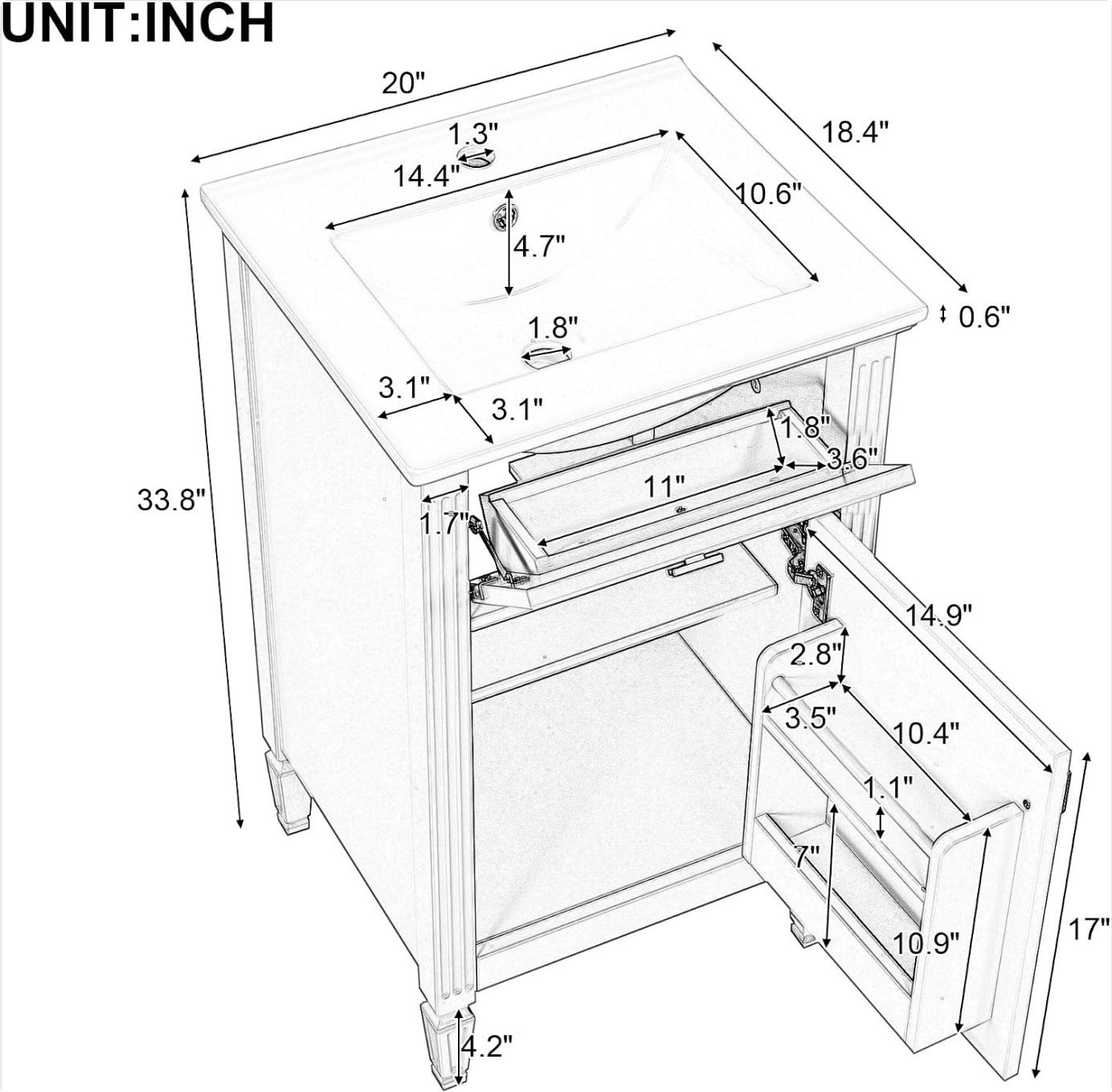
Image: External dimensions of the vanity, showing overall width (20 inches), depth (18.4 inches), and height (33.8 inches).
