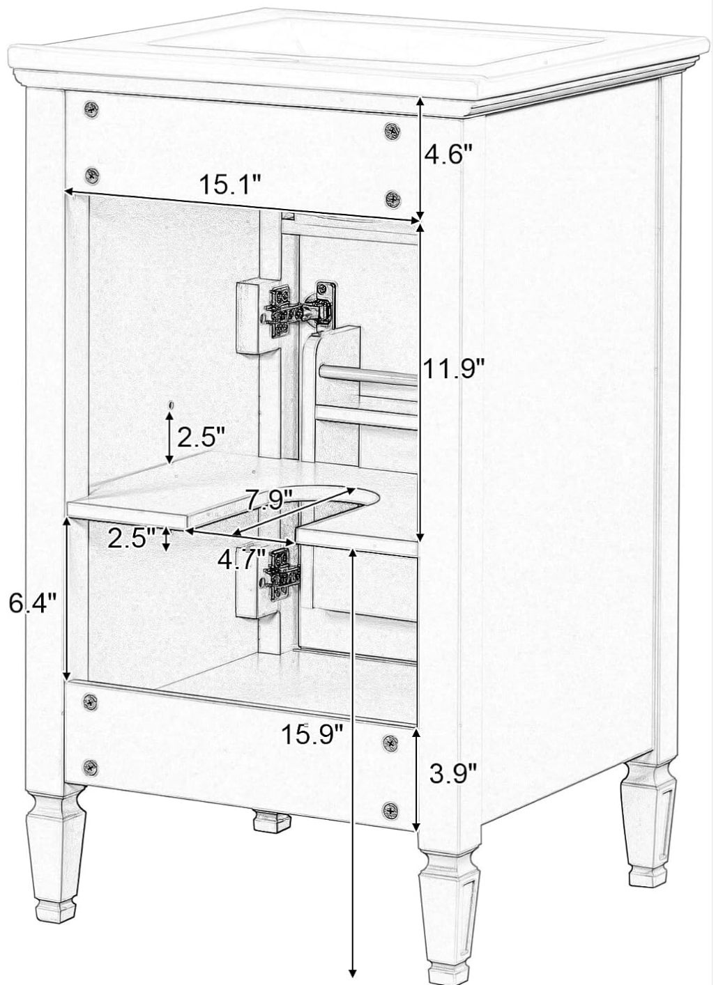
Image: Internal dimensions of the vanity cabinet, including shelf and plumbing cutout areas.
