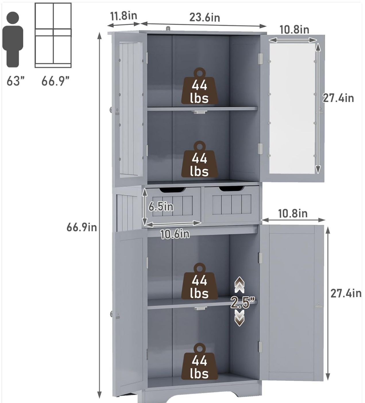
Image 4.1: Dimensional diagram of the cabinet, indicating overall height of 66.9 inches, width of 23.6 inches, and depth of 11.8 inches, along with internal shelf and drawer dimensions.
