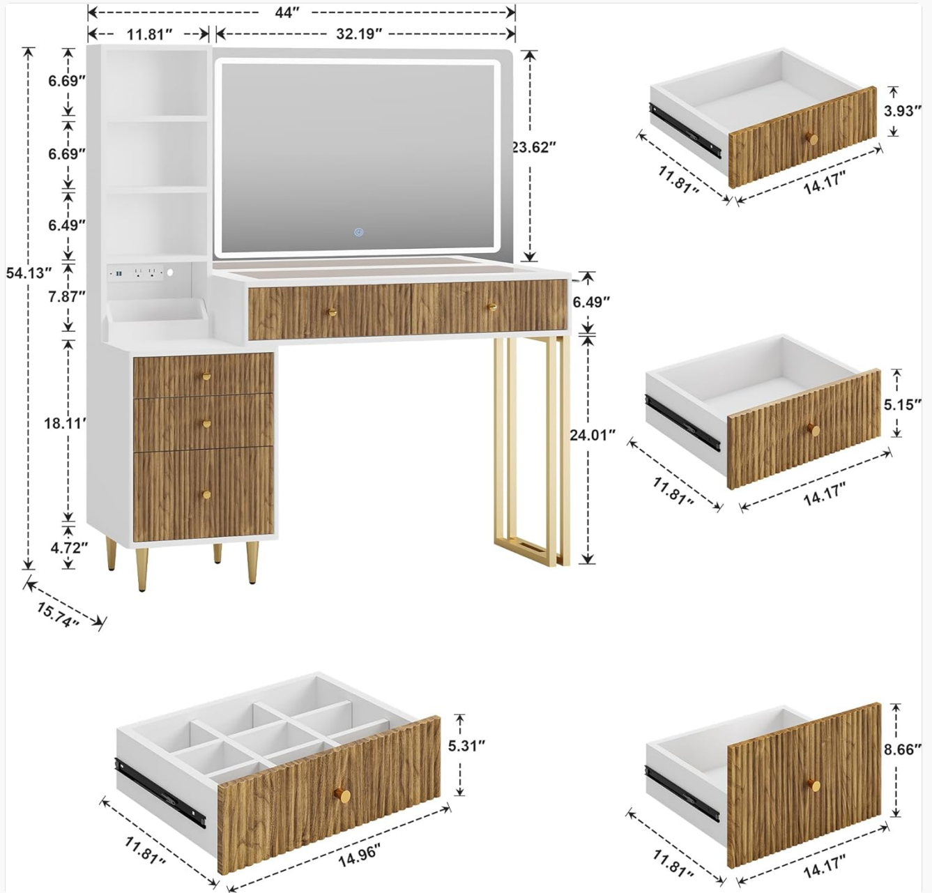
Figure 1: Overview of vanity desk components and dimensions. This diagram illustrates the various sections of the desk, including the mirror, shelves, drawers, and overall measurements, which are 15.74"D x 44"L x 54.13"H.
