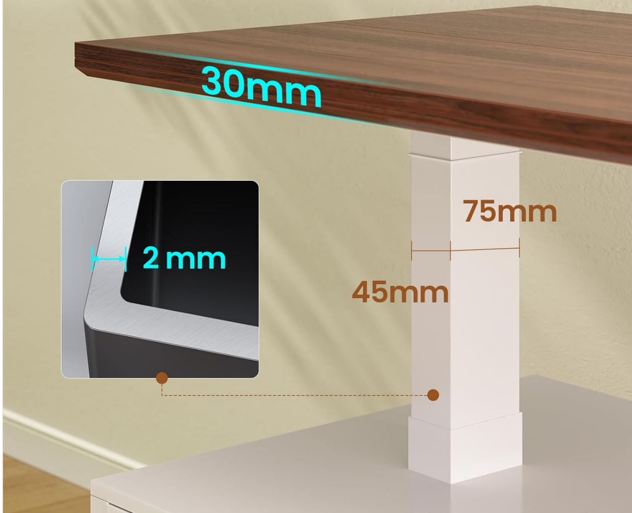
Figure 6.1: Details on the desk's robust construction, including 30mm thicker panel, 75mm x 45mm sturdy frame, and 9mm thicker storage cabinet for enhanced durability and stability.
