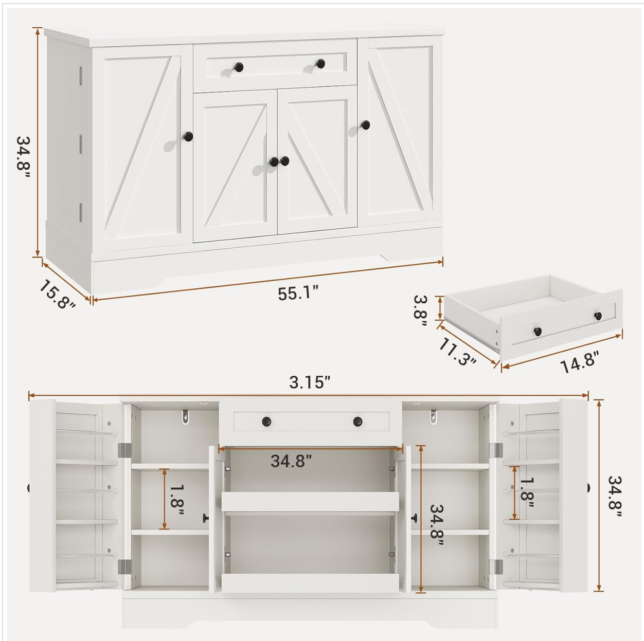
Image: Dimensional drawing of the buffet cabinet, providing key measurements for planning placement.
