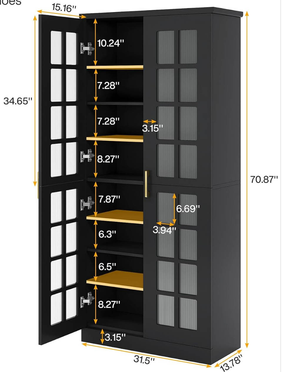
Image 2: Product dimensions and adjustable shelf details. The orange boards indicate movable shelves that can be removed to create taller compartments.
