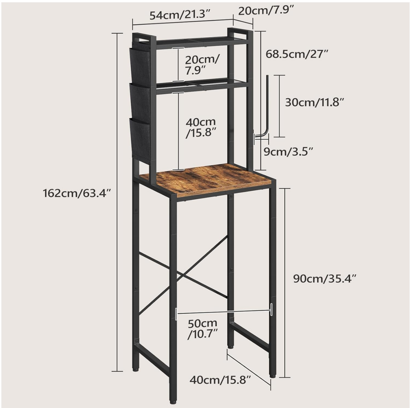
Image 4.2: Bakers Rack dimensions, including shelf heights and mini fridge compartment size.
