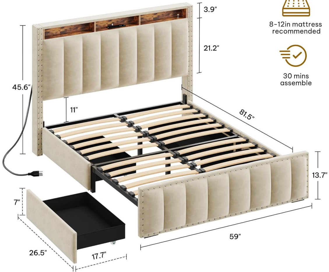
Image 3.1: Detailed dimensions of the bed frame, including headboard height, bed length, and width.
