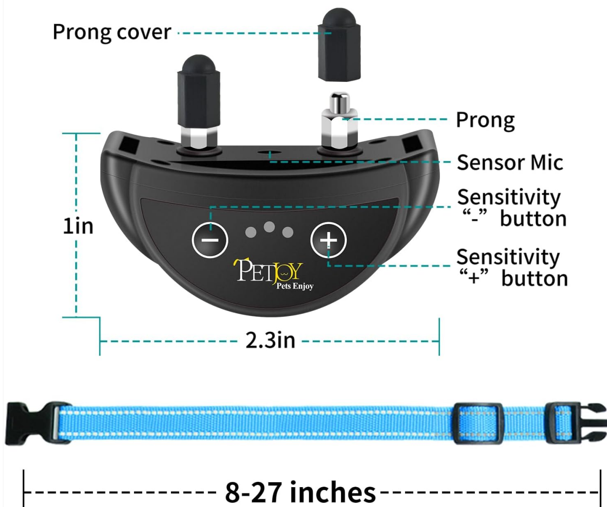
Figure 4.1: Collar Components and Dimensions. This diagram labels the prong cover, prong, sensor mic, and sensitivity buttons (+ and -) on the collar unit, along with its dimensions (1 inch height, 2.3 inches width) and the adjustable collar strap length (8-27 inches).
