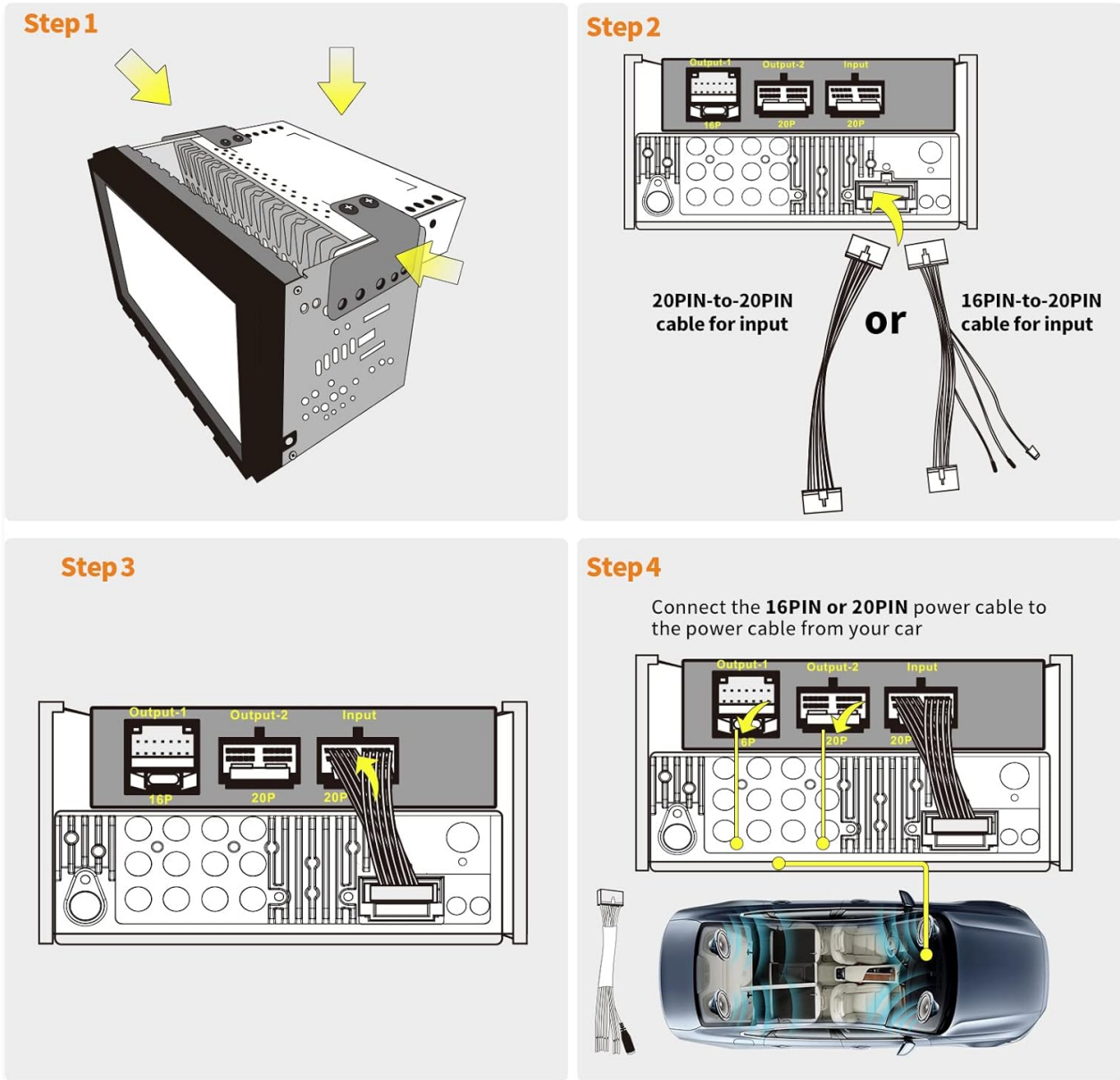
Image 4.1: Step-by-step visual guide for connecting the ATOTO amplifier to the head unit and the car's power system.
