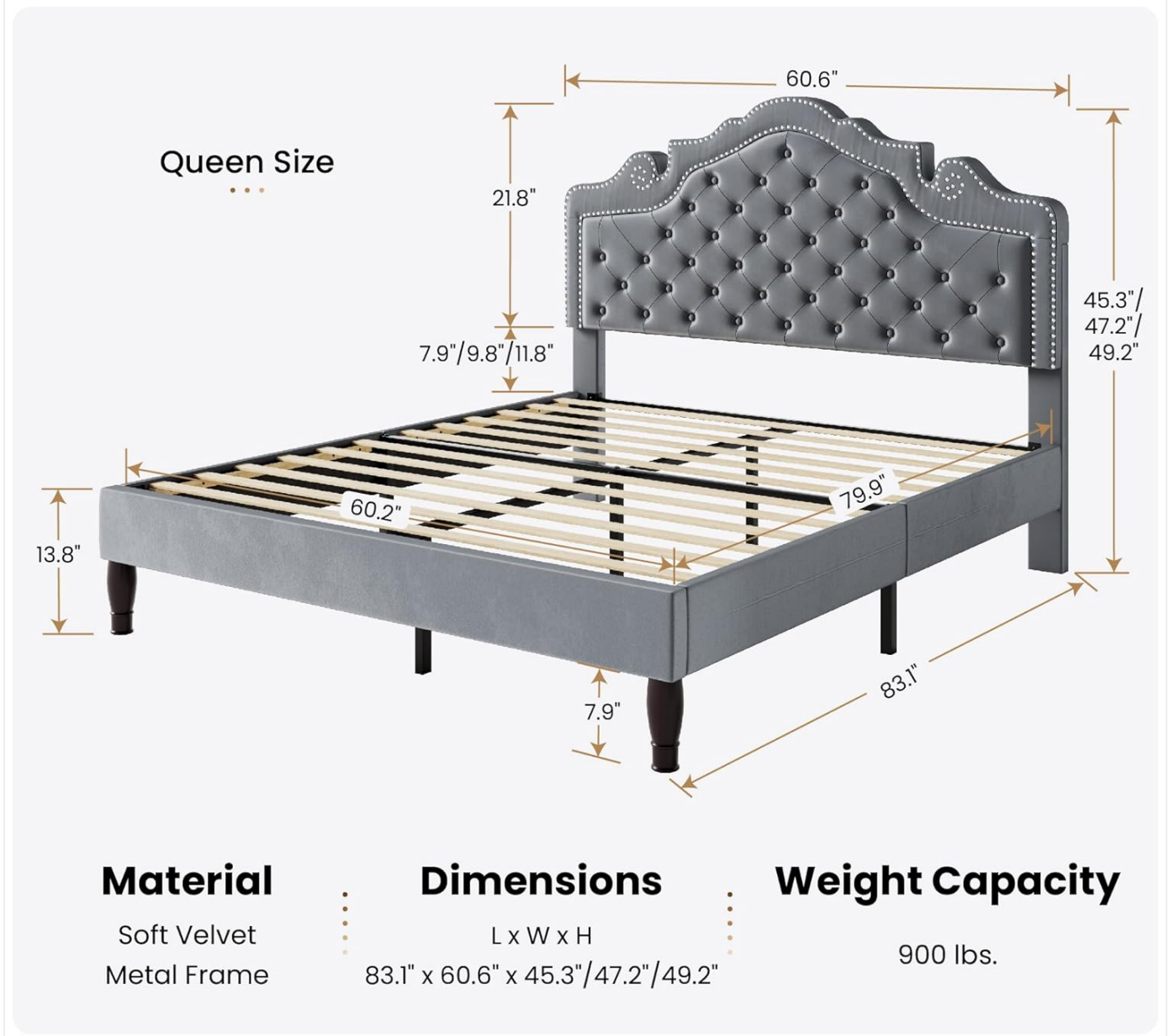
Figure 5: Product Information and Dimensions. This diagram provides precise measurements for the Queen size bed frame, including length, width, height, and under-bed clearance, along with material and weight capacity details.
