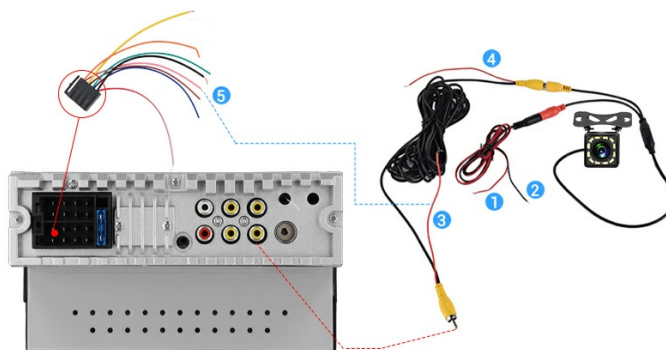
Image: A visual guide demonstrating the correct wiring for connecting the backup camera to the car stereo.
