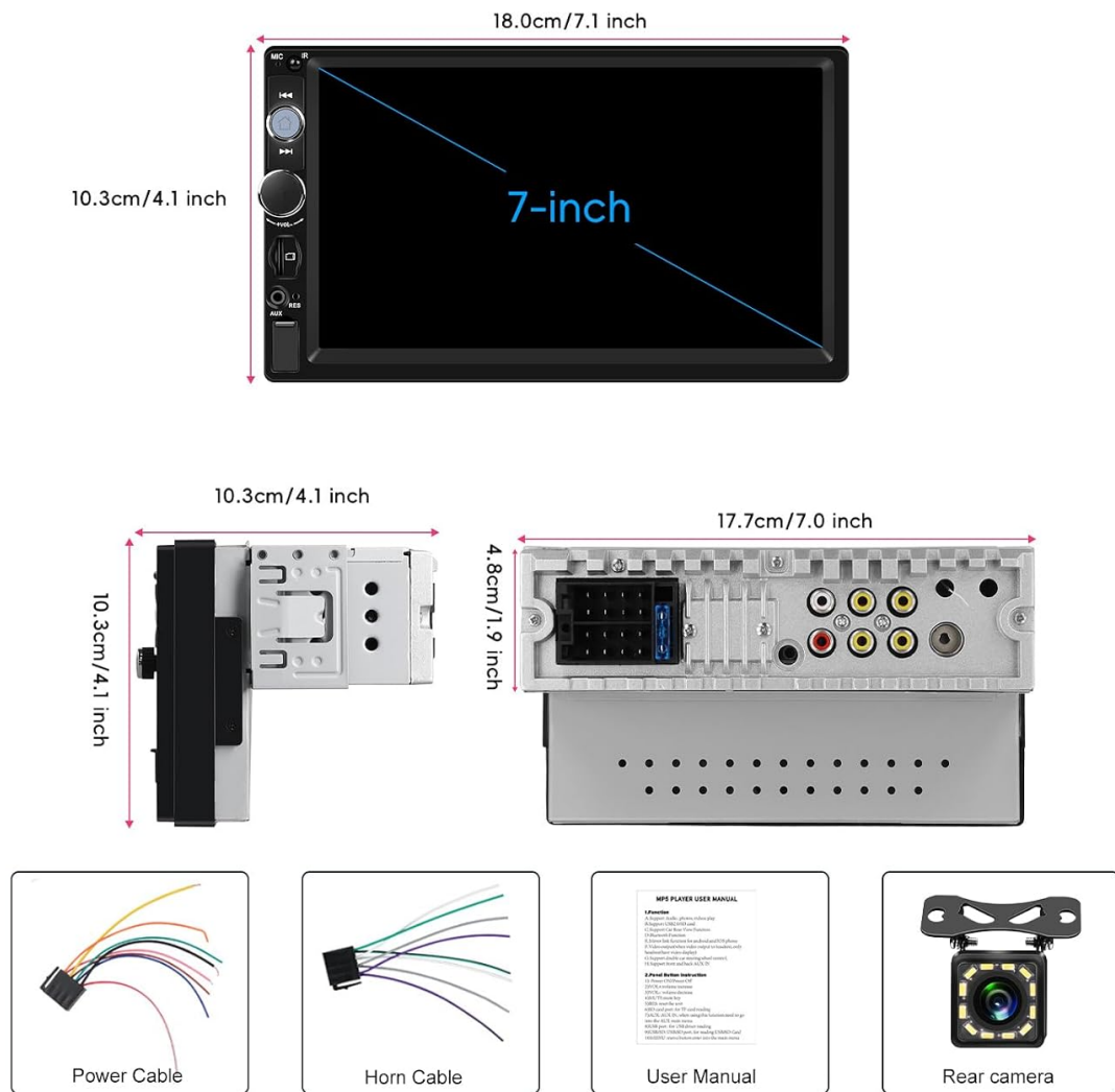
Image: An illustration detailing the dimensions of the car stereo and its included accessories, such as the power cable, horn cable, user manual, and rear camera.
