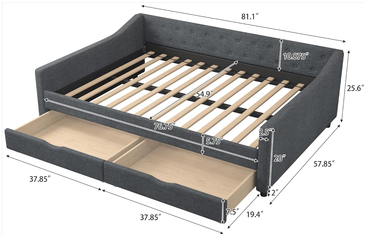
Image: A diagram illustrating the overall dimensions and key measurements of the daybed frame, including the storage drawers.
