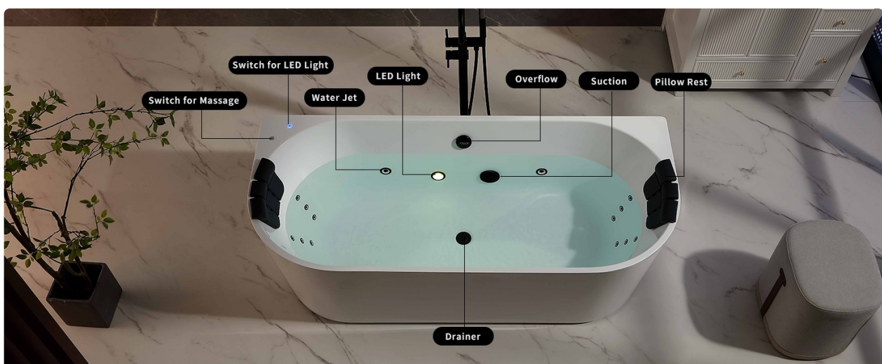
Image: Diagram showing the location of the massage switch, LED light switch, water jets, overflow, suction, pillow rest, and drain.
