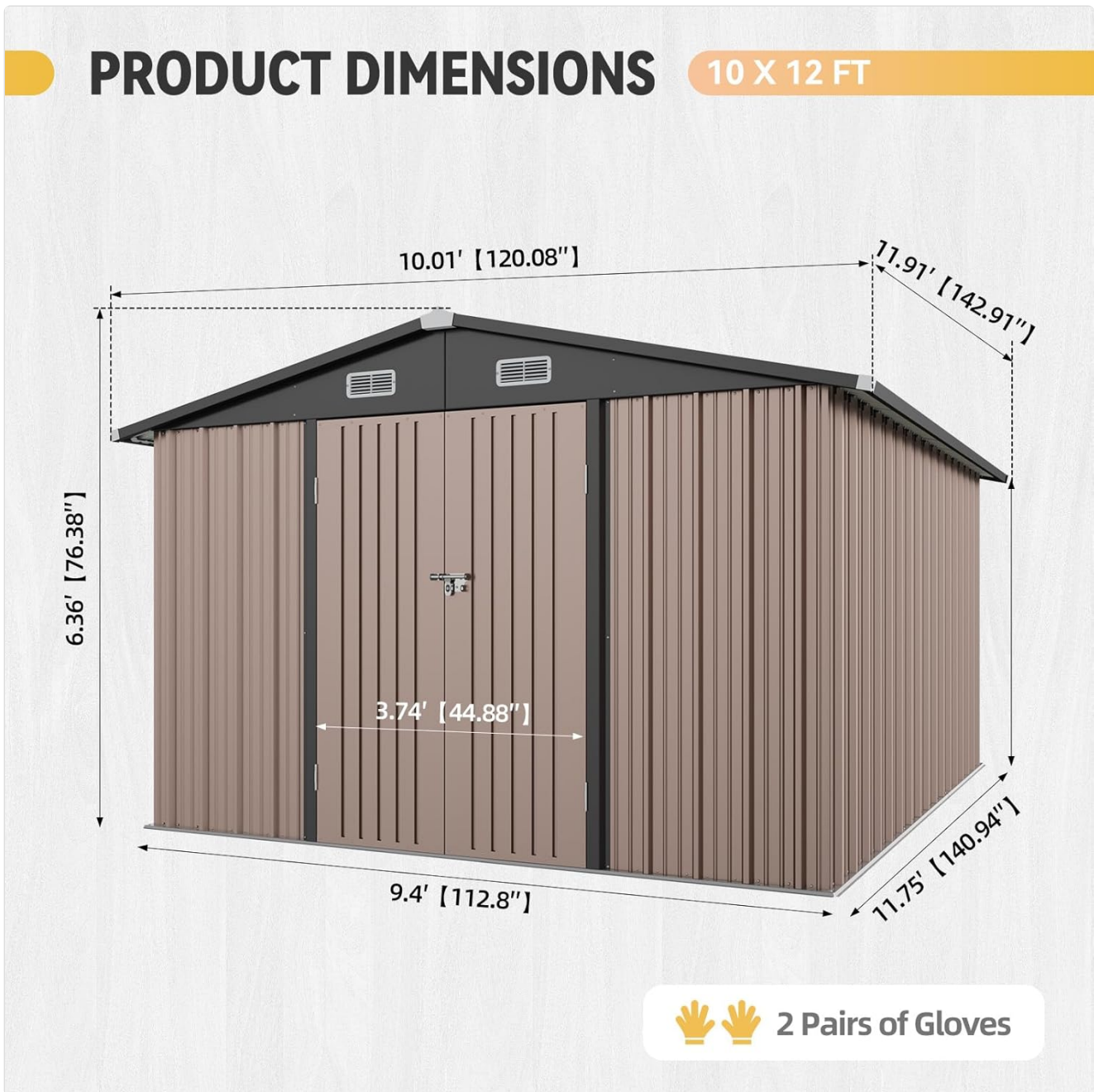
Figure 2: Detailed product dimensions for planning your installation space.
