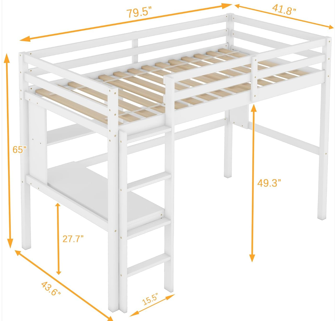
Image 4.1: Dimensional diagram of the loft bed, illustrating overall length, width, and height.
