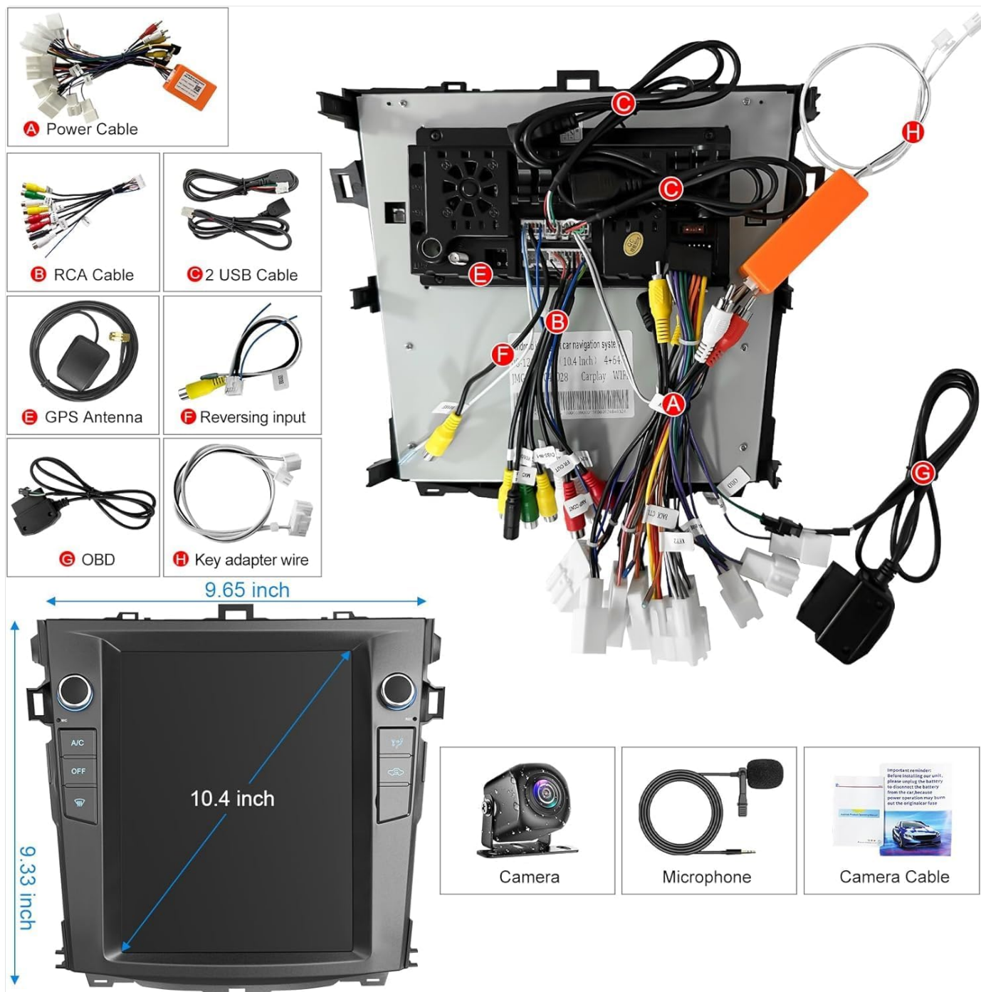
Figure 2.1: Included components and wiring diagram.
