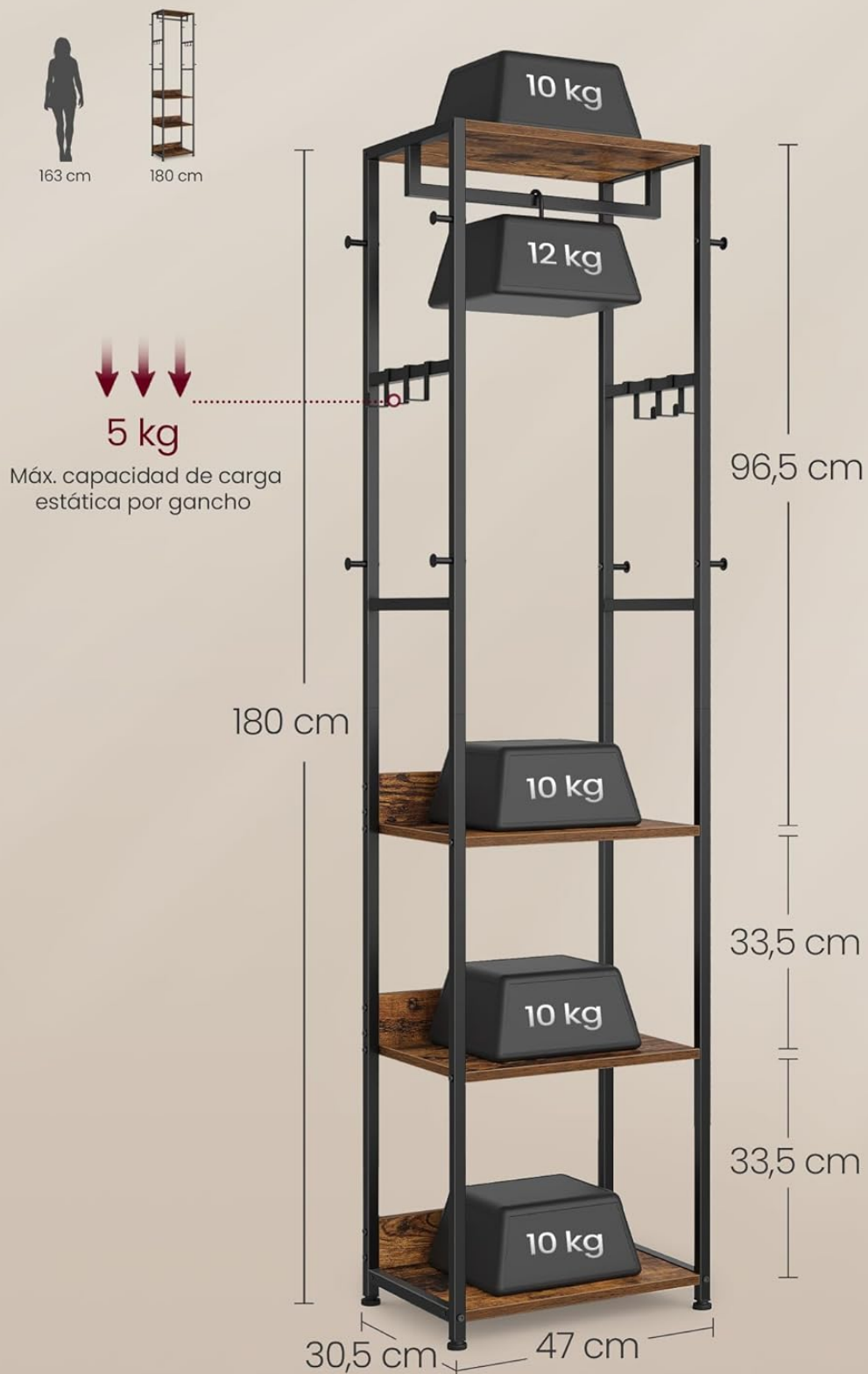
Image 4.2: Dimensional diagram and load capacities: 180 cm height, 47 cm width, 30.5 cm depth. Each shelf supports 10 kg, each hook 5 kg, with a total capacity of 100 kg.
