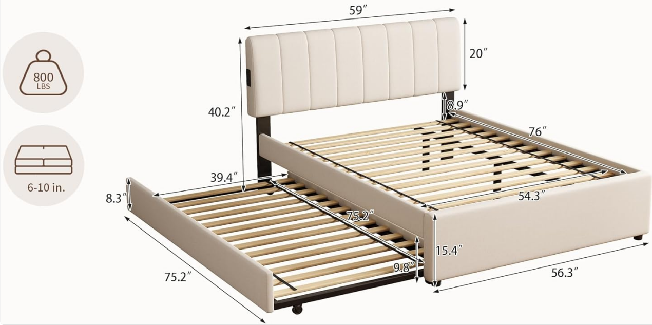
Figure 1: This diagram illustrates the key dimensions of the main bed frame and the pull-out trundle, including length, width, height, and recommended mattress thickness.
