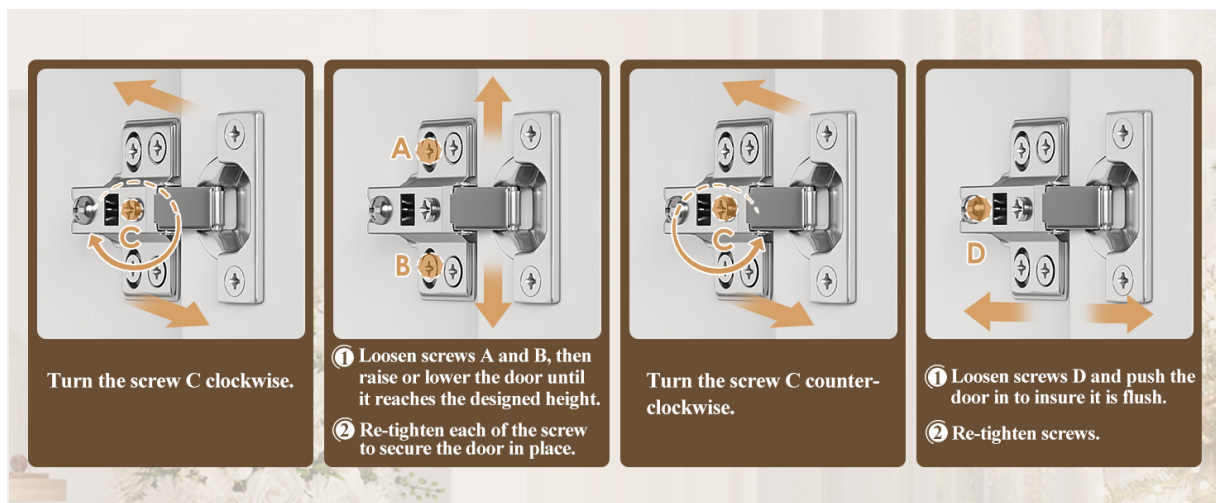
Figure 6.1: Visual guide for identifying and correcting common door alignment issues using hinge adjustments.
