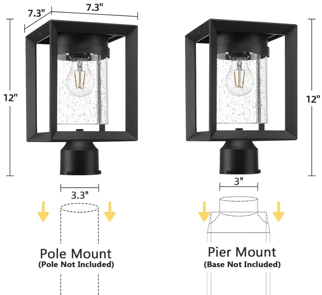
Figure 2: Pole mount and pier mount options. Compatible with 3.3-inch pole or 3-inch post mount base (not included).
