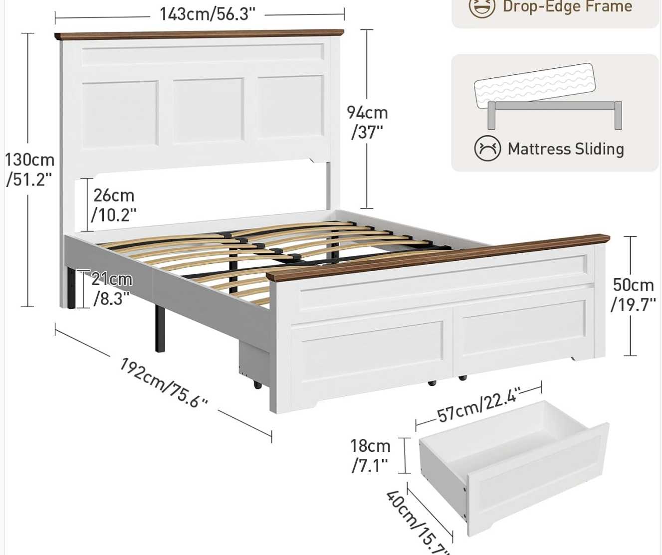
Image 5.1: Diagram illustrating the bed frame dimensions and the drop-edge frame feature to prevent mattress sliding.
