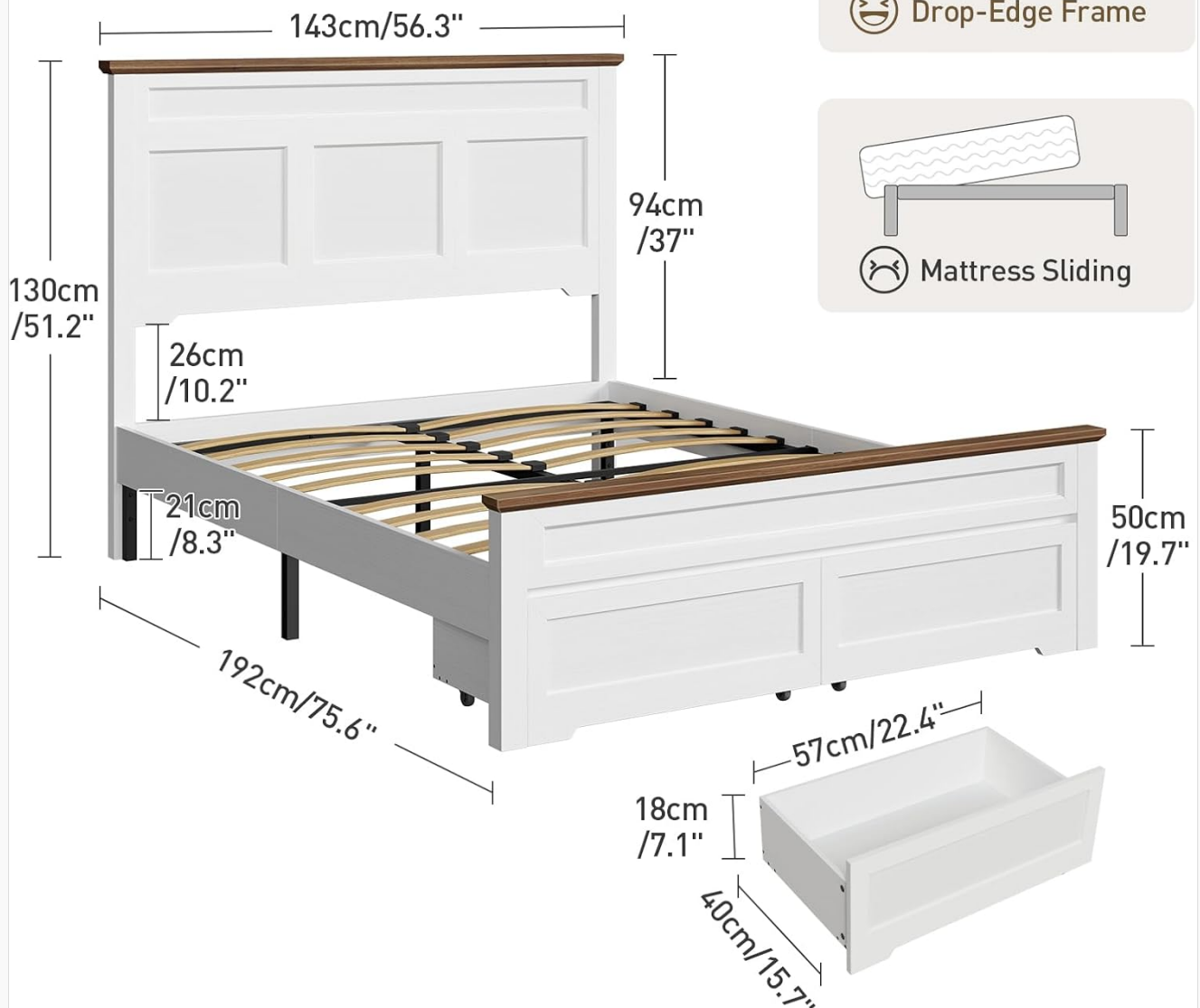
Image 8.1: Detailed diagram showing all key dimensions of the bed frame.
